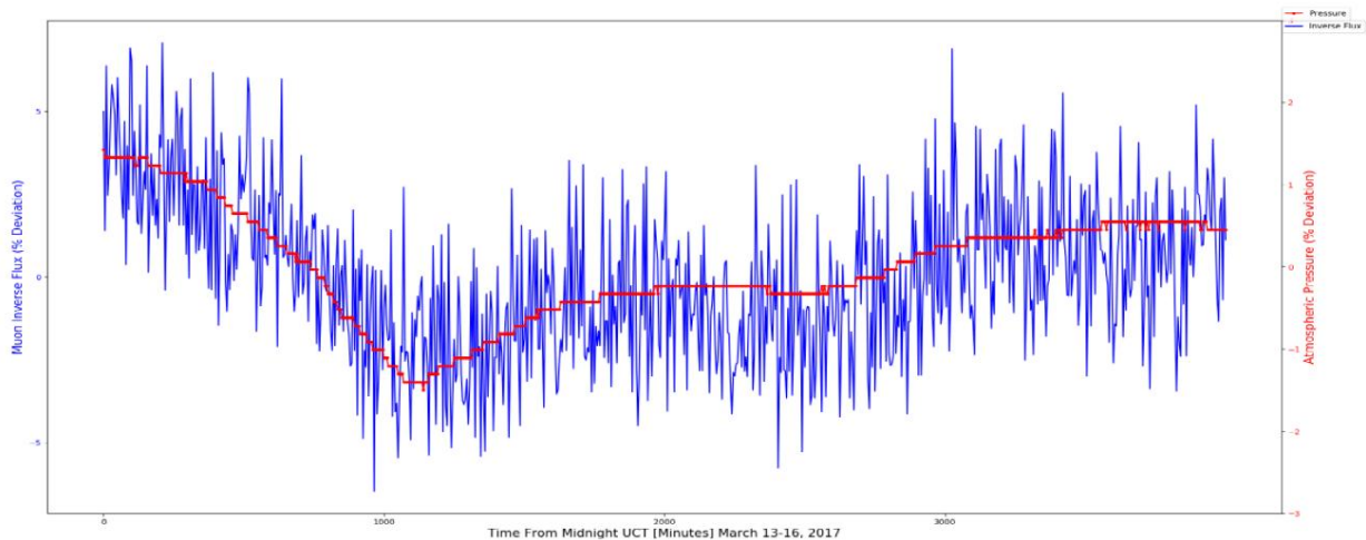
Figure 7: Inverse cosmic ray muon flux measurements (blue) overlaid with atmospheric pressure measurements (red); data recorded at Queensborough Community College using three QuarkNet detectors during winter storm "Stella" in March of 2017.
